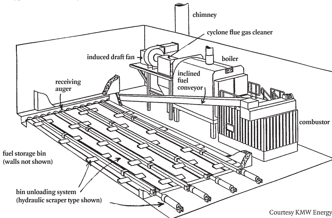
Figure 3.1 A Typical Biomass System
